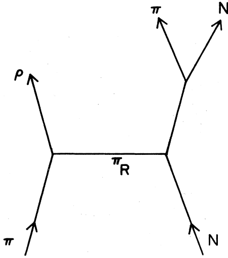
FIG. 20. Tree graphs included in a Steinmann-obeying model for \pi N \rightarrow \rho\pi N with s -channel helicity conservation for the subprocess \pi_R N \rightarrow \pi N .
